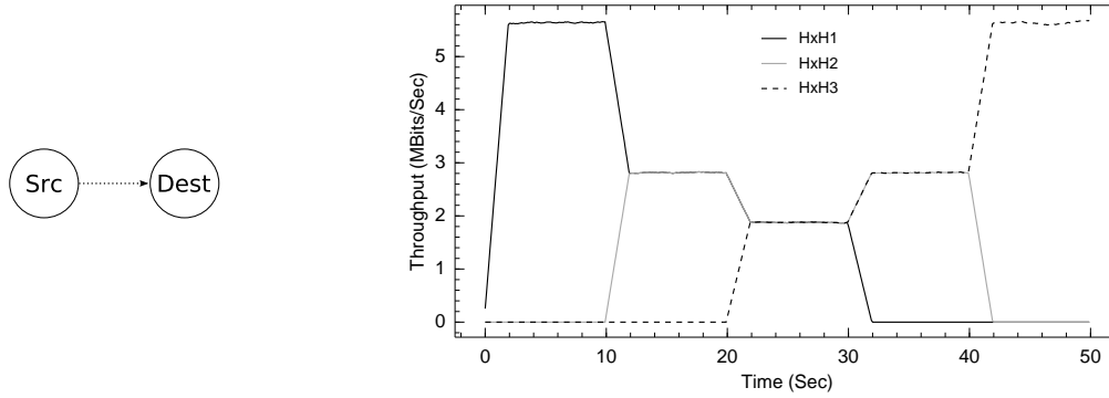
Figure 4.1: Control Topology (Left) : The simplest case for a hop-by-hop protocol is a single pair of nodes. Results (Right) : As expected, the scheduler is able to distribute bandwidth between various flows traversing a node.
