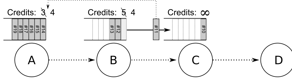
Figure 3.3: Passive Credit Management : Each time a node sends a packet, it decrements its credit count. The packet is overheard upstream, allowing nodes to increment their credit count without sending explicit messages.
